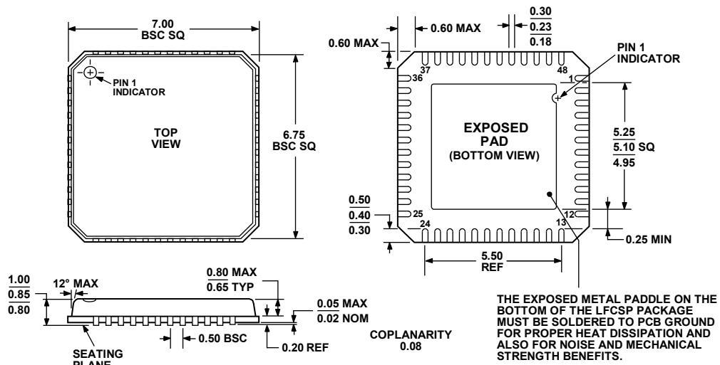
Figure 37. 48-Lead Lead Frame Chip Scale Package [LFCSP_VQ] 7 mm × 7 mm Body, Very Thin Quad (CP-48-1)
