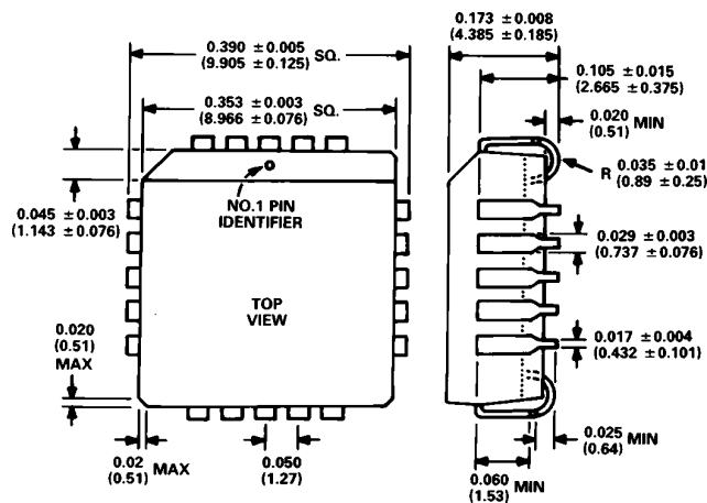
20-Terminal Plastic Leaded Chip Carrier (P-20A)
