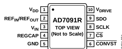
Figure 4. Pin Configuration, 10-Lead MSOP
