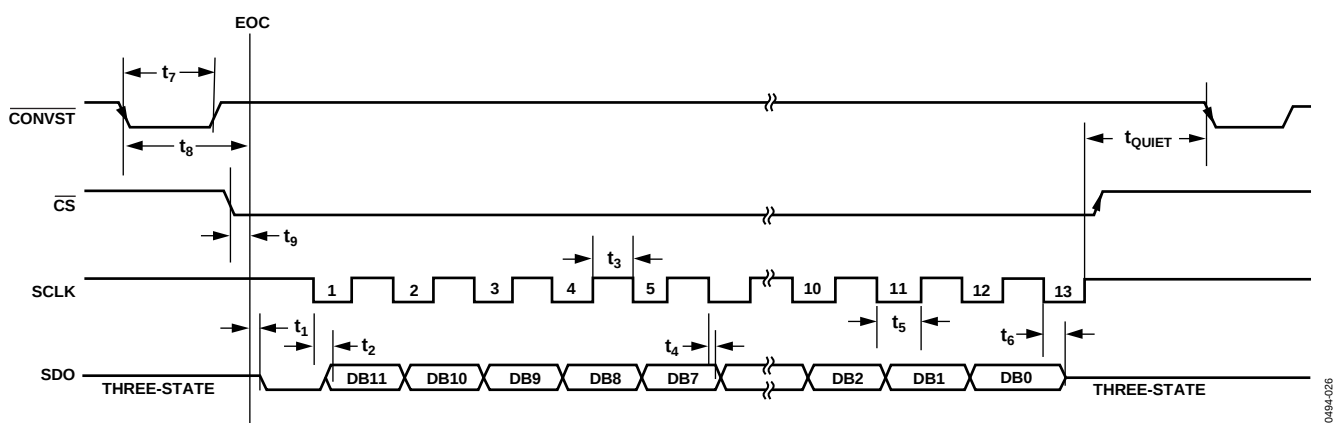
Figure 27. Serial Port Timing with BUSY Indicator
