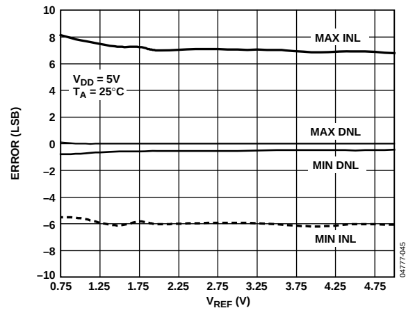
Figure 8. INL and DNL Error vs. V_{REF}
