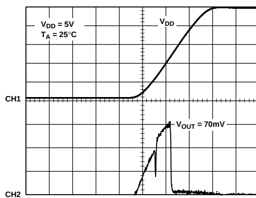
Figure 25. Power-On Reset to 0 V
