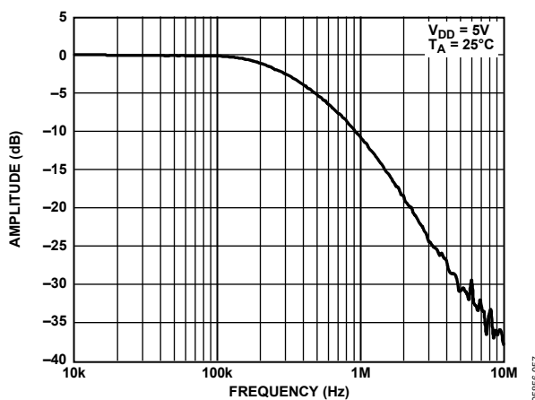
Figure 49. Multiplying Bandwidth
