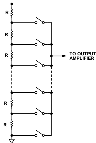
Figure 51. Resistor String
