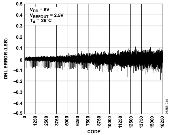
Figure 14. AD5644R-5 DNL, Internal Reference
