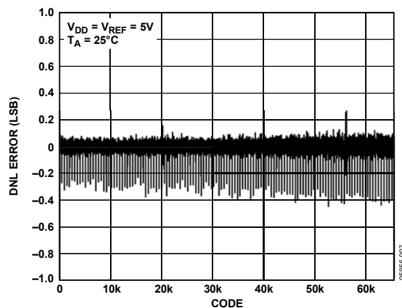
Figure 7. AD5664R DNL, External Reference
