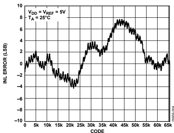
Figure 4. AD5664R INL, External Reference
