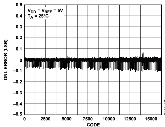
Figure 8. AD5644R DNL, External Reference
