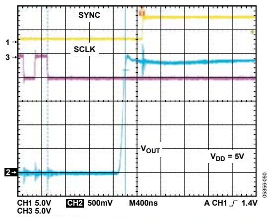
Figure 39. Exiting Power-Down to Midscale
