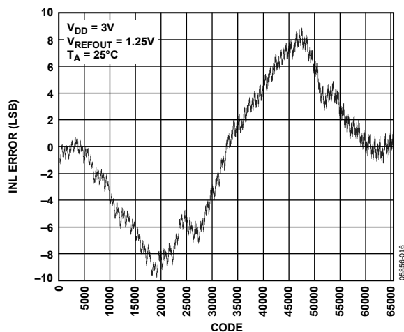
Figure 16. AD5664R-3 INL, Internal Reference
