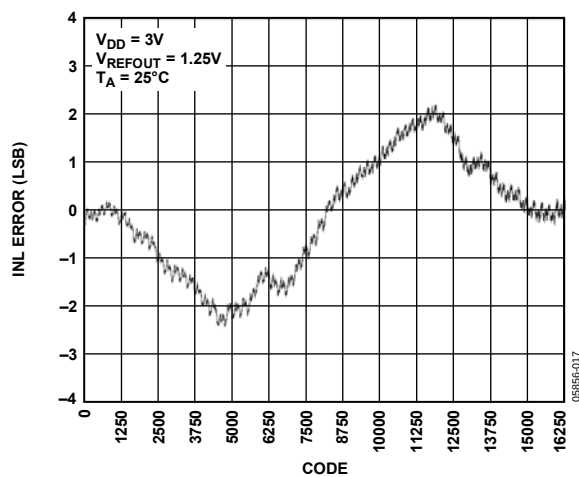
Figure 17. AD5644R-3 INL, Internal Reference
