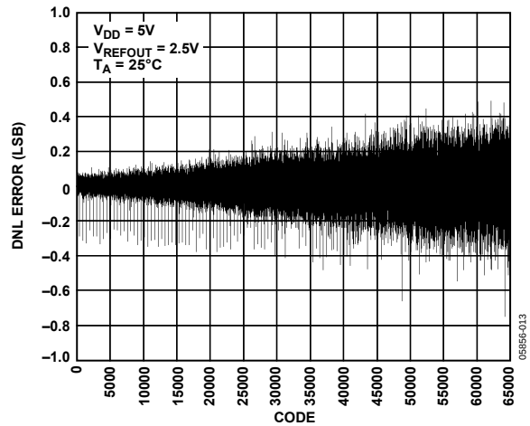
Figure 13. AD5664R-5 DNL, Internal Reference
