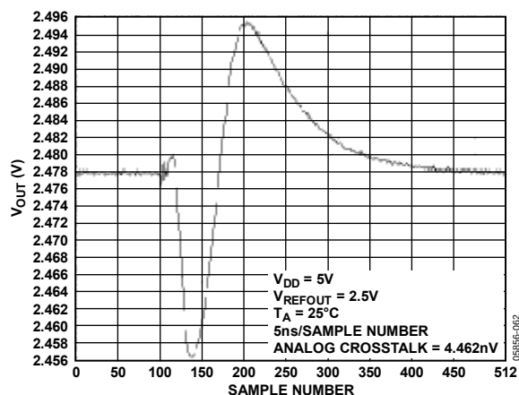
Figure 42. Analog Crosstalk, 2.5 V Internal Reference
