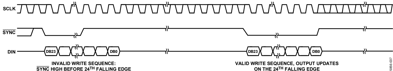
Figure 55. \overline{\text{SYNC}} Interrupt Facility
