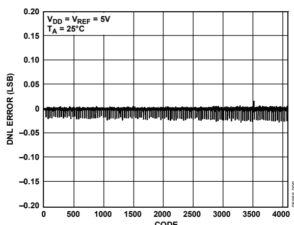
Figure 9. AD5624R DNL, External Reference
