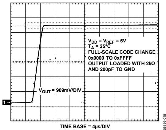
Figure 37. Full-Scale Settling Time, 5 V
