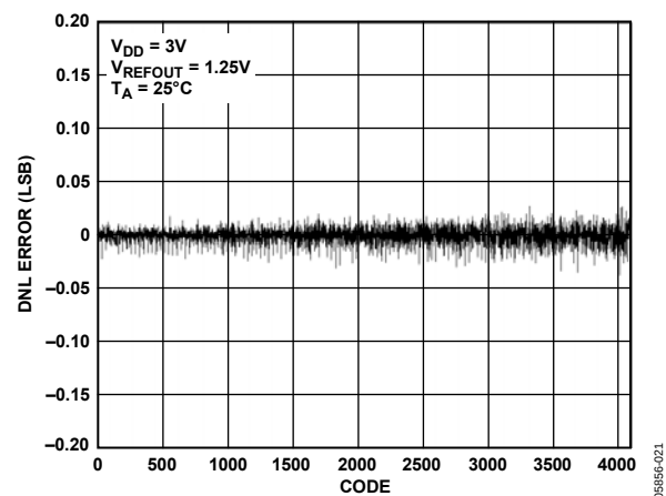
Figure 21. AD5624R-3 DNL, Internal Reference
