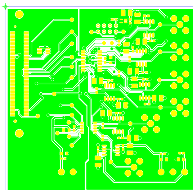
Figure 34. Component Side
