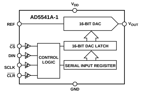
Figure 2. AD5541A-1
