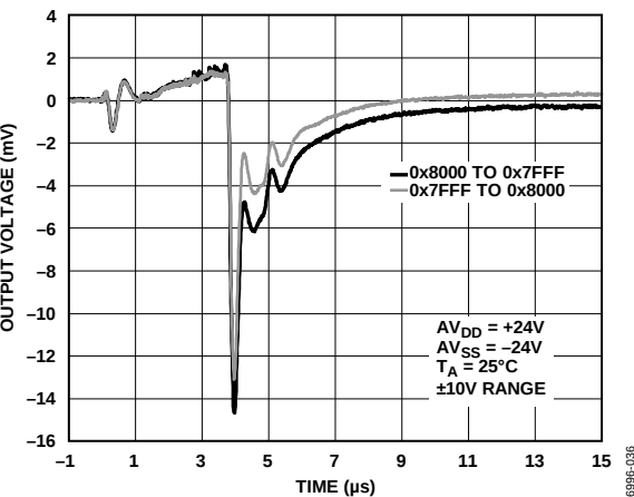
Figure 38. Digital-to-Analog Glitch
