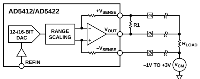
Figure 65. Voltage Output
