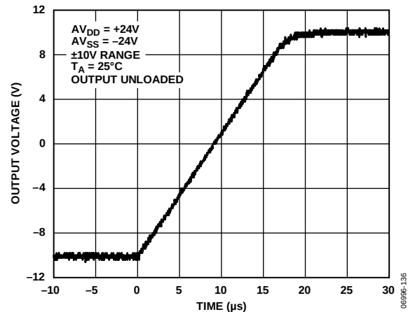
Figure 36. Full-Scale Positive Step
