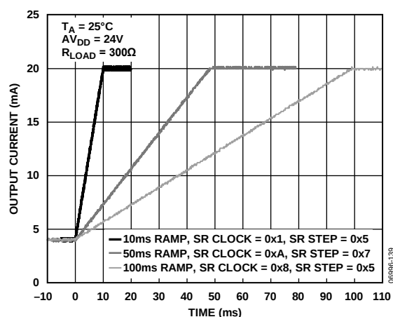
Figure 68. Output Current Slewling Under Control of the Digital Slew Rate Control Feature
