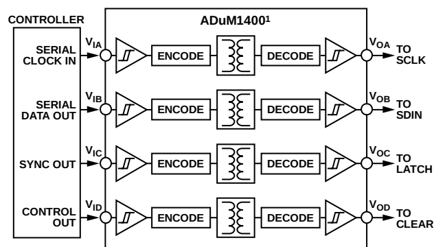
Figure 74. Isolated Interface
