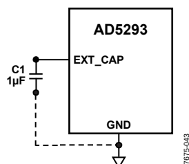
Figure 49. Hardware Setup for the EXT_CAP Pin
