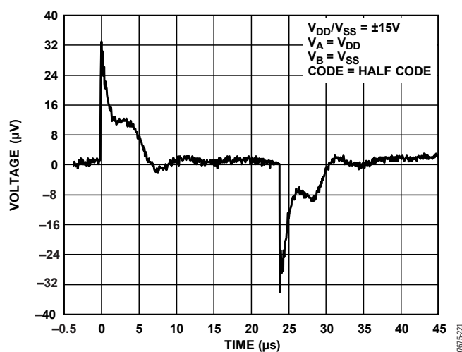
Figure 35. Digital Feedthrough
