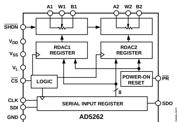
Figure 2. AD5262
