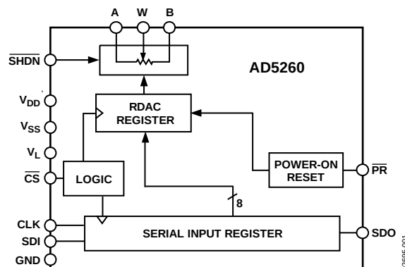
Figure 1. AD5260
