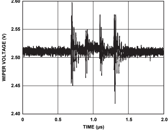
Figure 25. Digital Feedthrough
