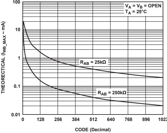
Figure 26. I_{WB\_MAX} vs. Code
