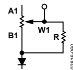
Figure 61. Resistor Scaling with Pseudo Log Adjustment Characteristics
