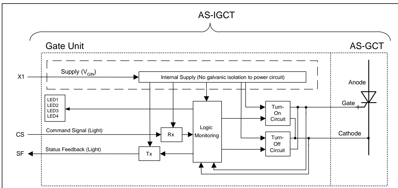
Fig. 13 Block diagram
