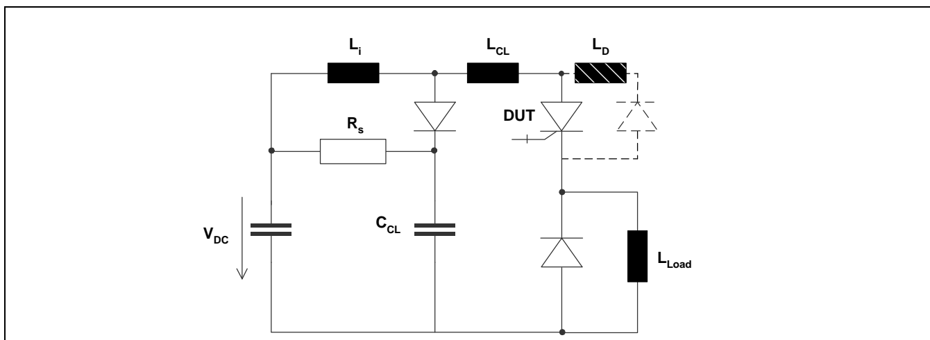
Fig. 15 Test circuit
