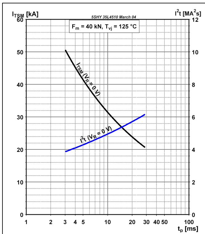
Fig. 5 Surge on-state current vs. pulse length. Half-sine wave.
