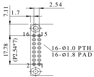
PIN DETAIL
