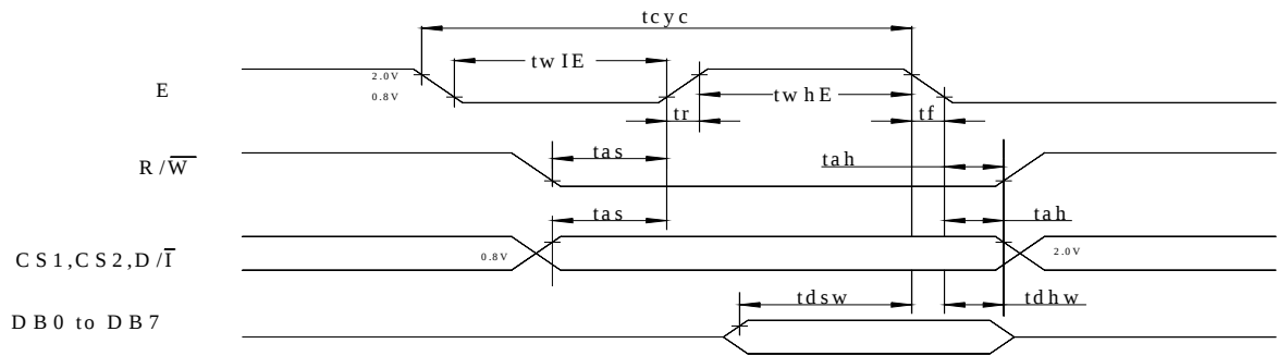
MPII Write Timing
