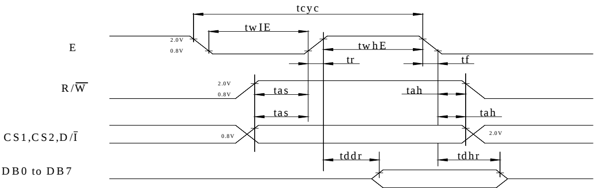
MPII Read Timing
