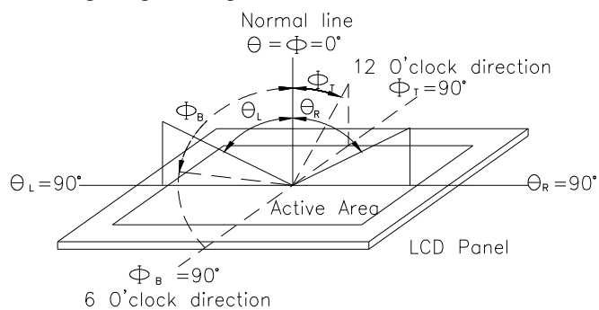
Fig. 7.1. Definition of viewing angle
