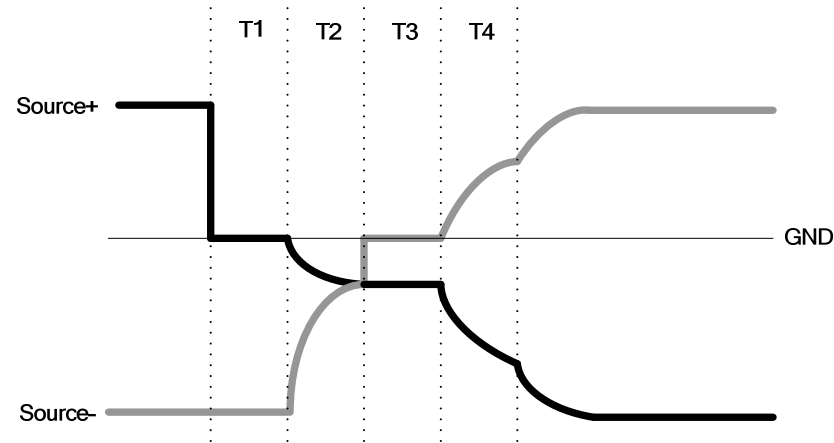
Source equalizing T4 time adjustment
