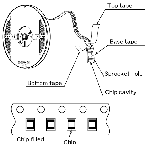
Card board carrier tape
