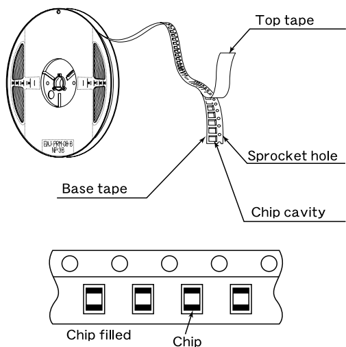
Embossed Tape
