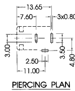
PIERCING PLAN
