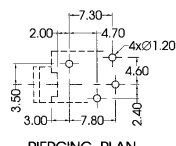
PIERCING PLAN
