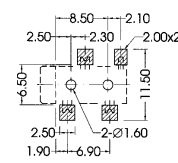
PIERCING PLAN
