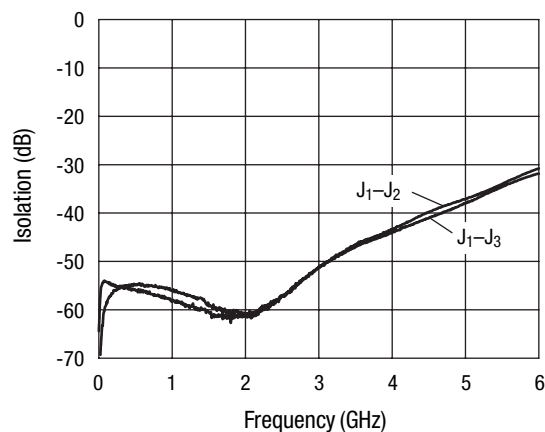
Isolation, 25 °C V_{DD} = 5 V, V_{CTL} = 0/5 V
