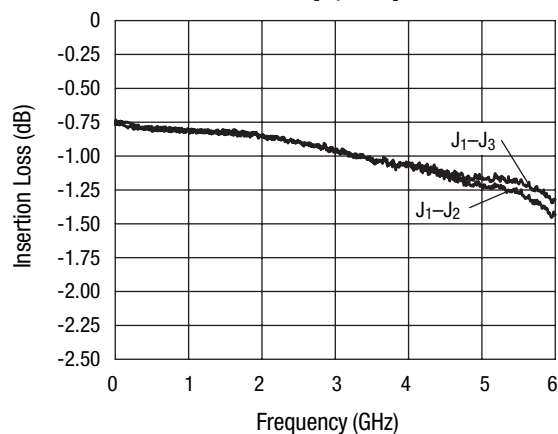
Insertion Loss, 25 °C V_{DD} = 5 V, V_{CTL} = 0/5 V
