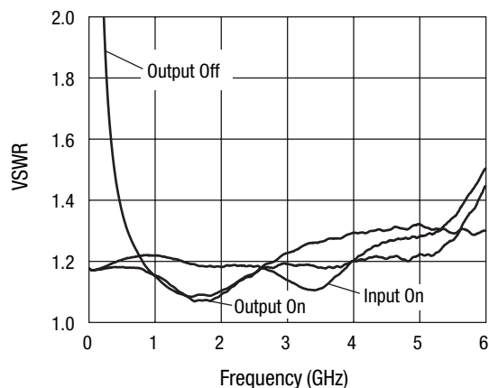
VSWR, 25 °C V_{DD} = 5 V, V_{CTL} = 0/5 V
