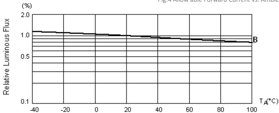
Fig.5 Luminous Intensity at I f =150Ma vs. Ambient Temperature
