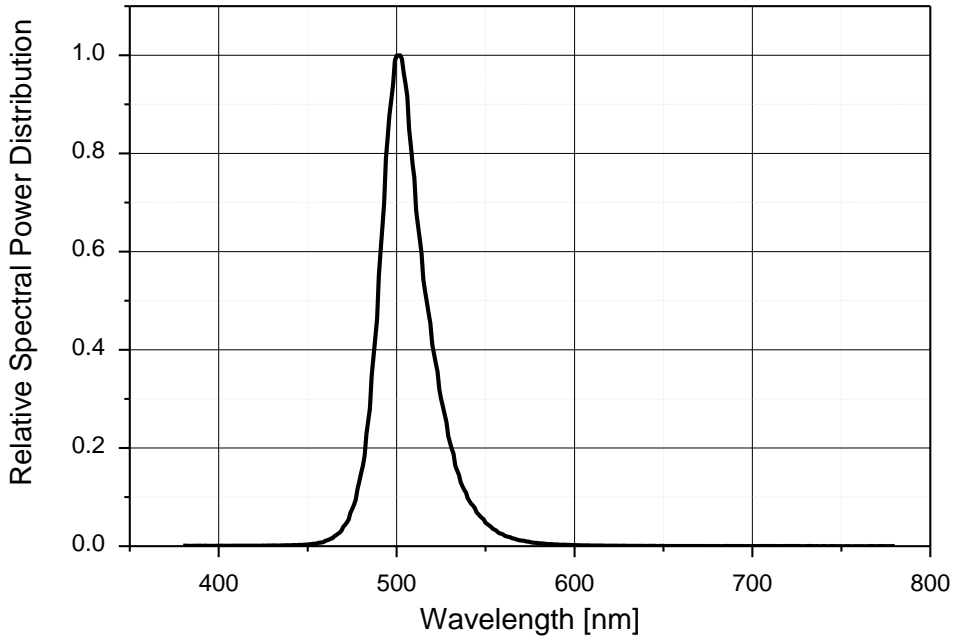
Color Spectrum (IF=350mA, Ta=25°C, RH30%)
