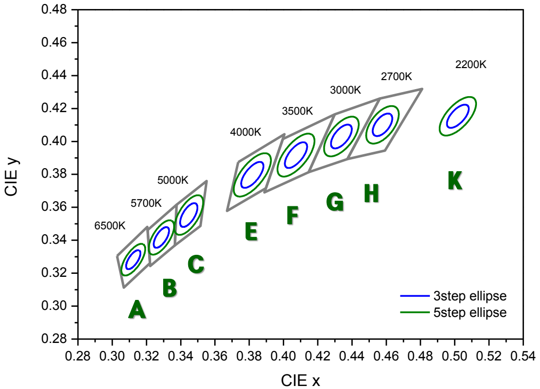
CIE Chromaticity Diagram T_j=85^\circ\text{C} , I_f=640\text{mA}
