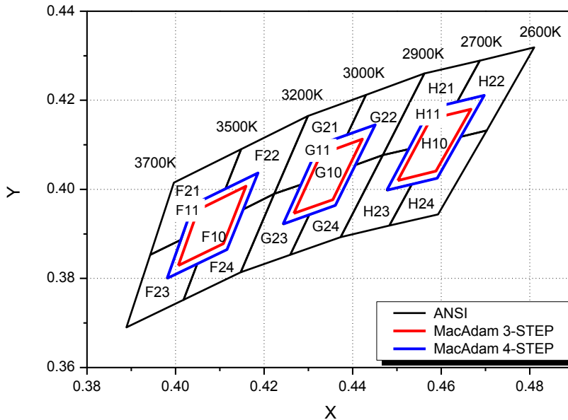
CIE Chromaticity Diagram, T_j=25^{\circ}\text{C} , I_f=1\text{A}
