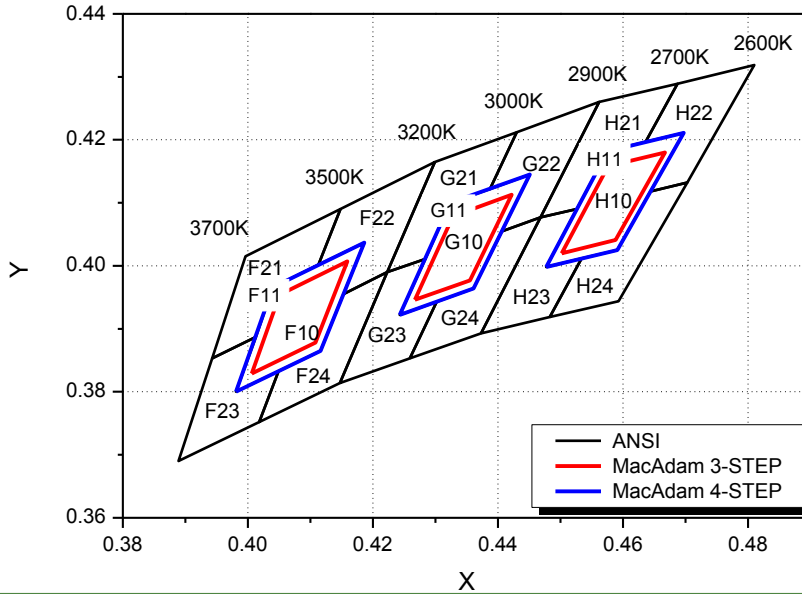
CIE Chromaticity Diagram, T_j=25^{\circ}\text{C} , I_f=700\text{mA}
