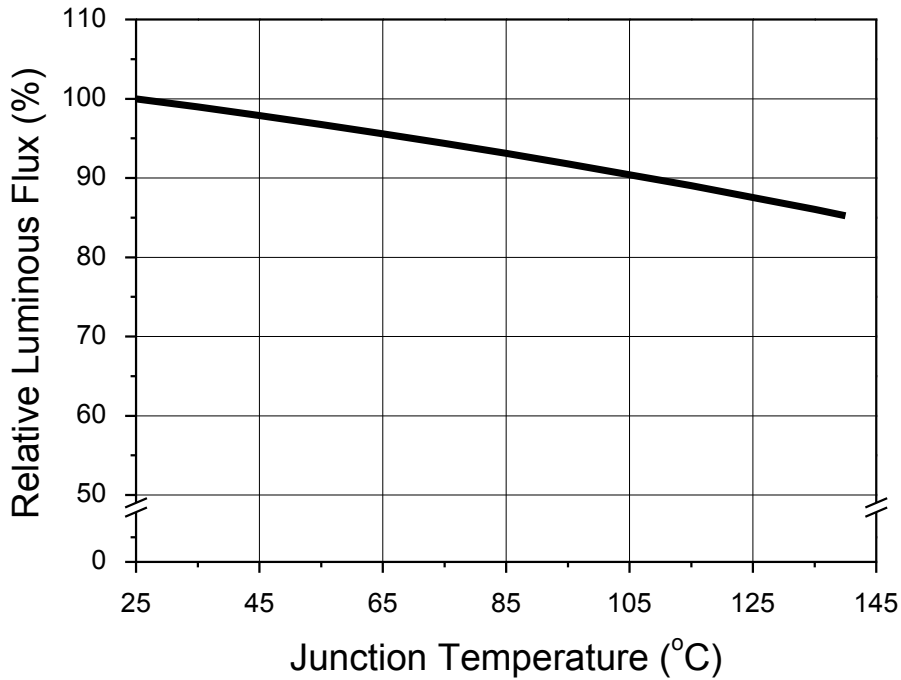
Fig 6. Junction Temperature vs. Relative Luminous Flux, I_F=0.72A
