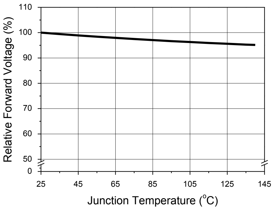
Fig 7. Junction Temperature vs. Forward Voltage, I_F=0.72A
