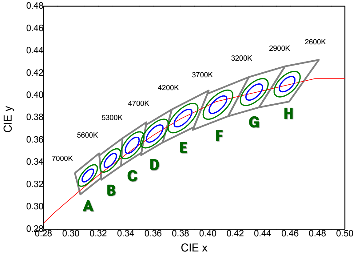
CIE Chromaticity Diagram T_j=25^\circ\text{C} , I_f=60\text{mA}
