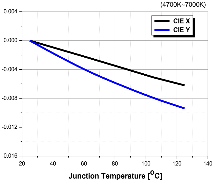
Fig 8. Junction Temp. vs. CIE X, Y Shift, I_F=60mA
