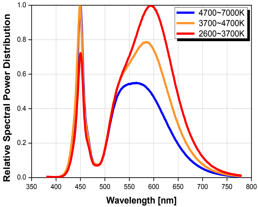
Fig 1. Color Spectrum, T_j=25^\circ\text{C} , I_F=60\text{mA}
