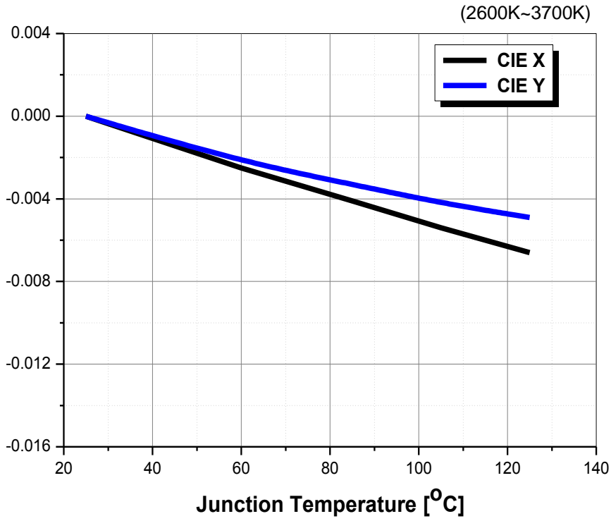
Fig 8. Junction Temp. vs. CIE X, Y Shift, I_F=60\text{mA}
