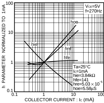
Fig.15 h parameter vs. collector current
