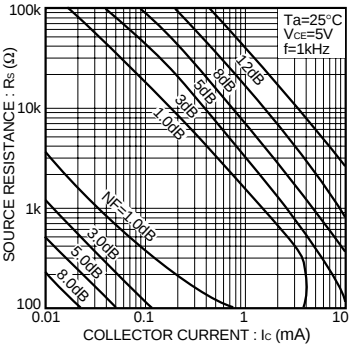
Fig.18 Noise characteristics (III)
