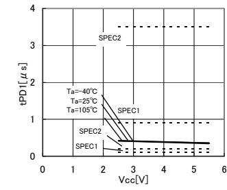
Fig.25 Output data delay time t_{PD1}
