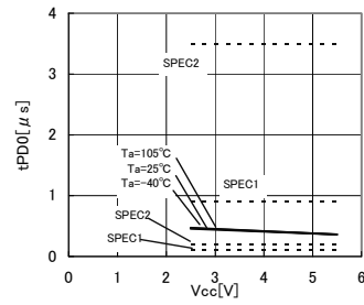
Fig.24 Output data delay time t_{PD0}
