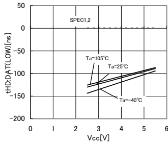
Fig.21 Input data hold time t_{HD:DAT(LOW)}
