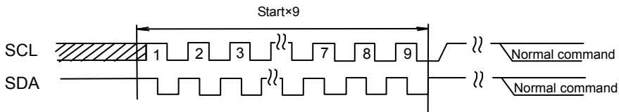
Fig.47-(c) START×9+ command input
