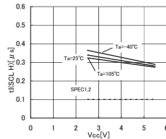
Fig.28 Noise removal valid time t(SCL H)
