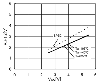
Fig.3 H input voltage V_{IH1,2} (SCL,SDA,WP)
