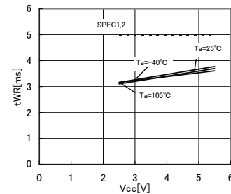
Fig.27 Internal write cycle time t_{WR}
