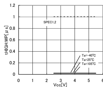
Fig.33 WP valid time t_{HIGH:WP}
