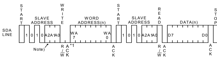
Fig.42 Random read cycle (BR24A01A/02/04/08/16-WM)
