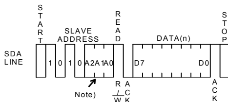
Fig.44 Current read cycle
