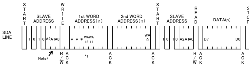
Fig.43 Random read cycle (BR24A32/64 -WM)
