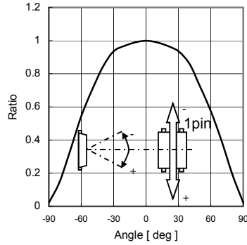
Fig.5 Directional Characteristics 2
