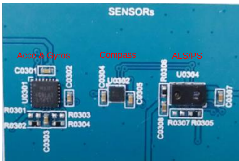
Figure 41: Sensors
