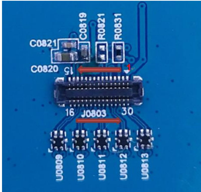
Figure 18: Pin Assignments of LCM Interfaces
