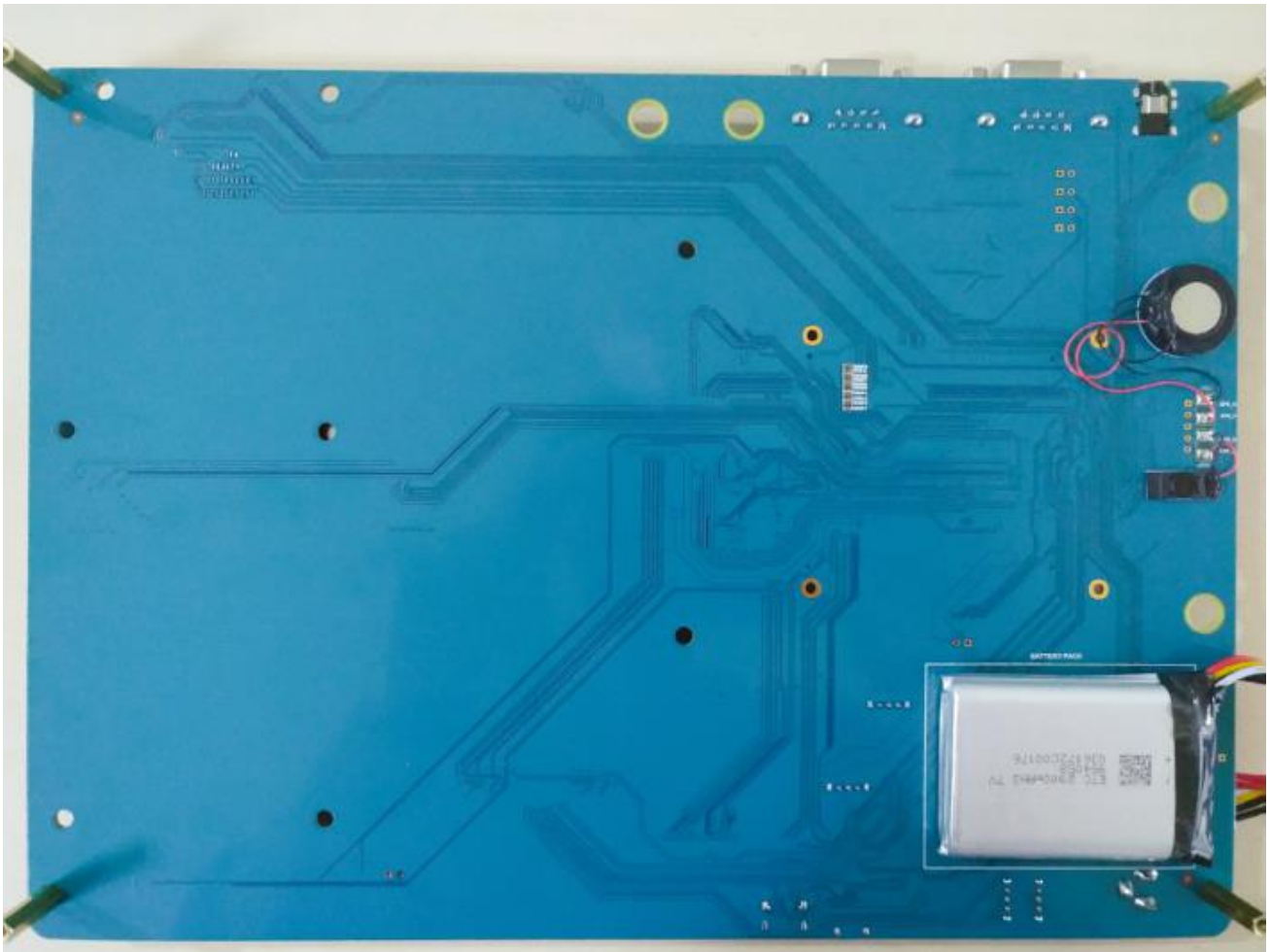
Figure 4: Smart EVB G2 Bottom View
