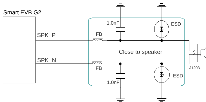
Figure 26: Reference Design for Loudspeaker Interface
