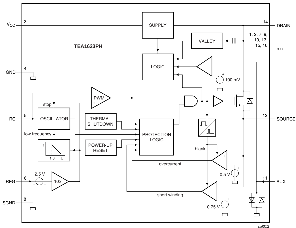
Fig 2. Block diagram of TEA1623PH
