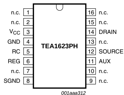
Fig 4. Pin configuration for SOT38-1 (DIP16)
