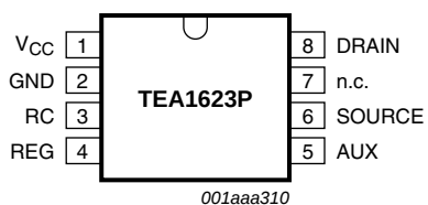
Fig 3. Pin configuration for SOT97-1 (DIP8)
