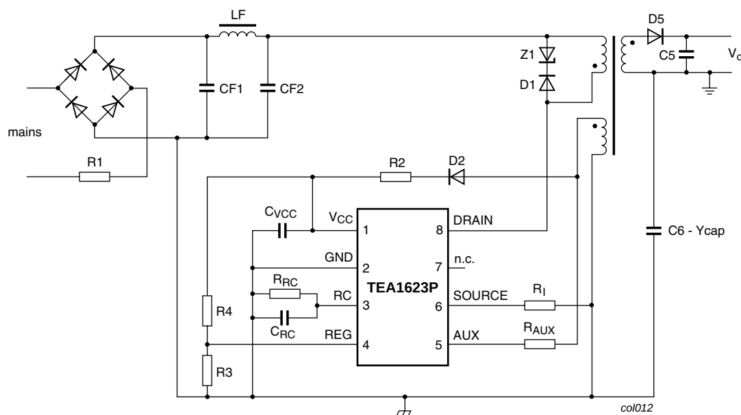
Fig 7. Application with primary sensing for TEA1623P
