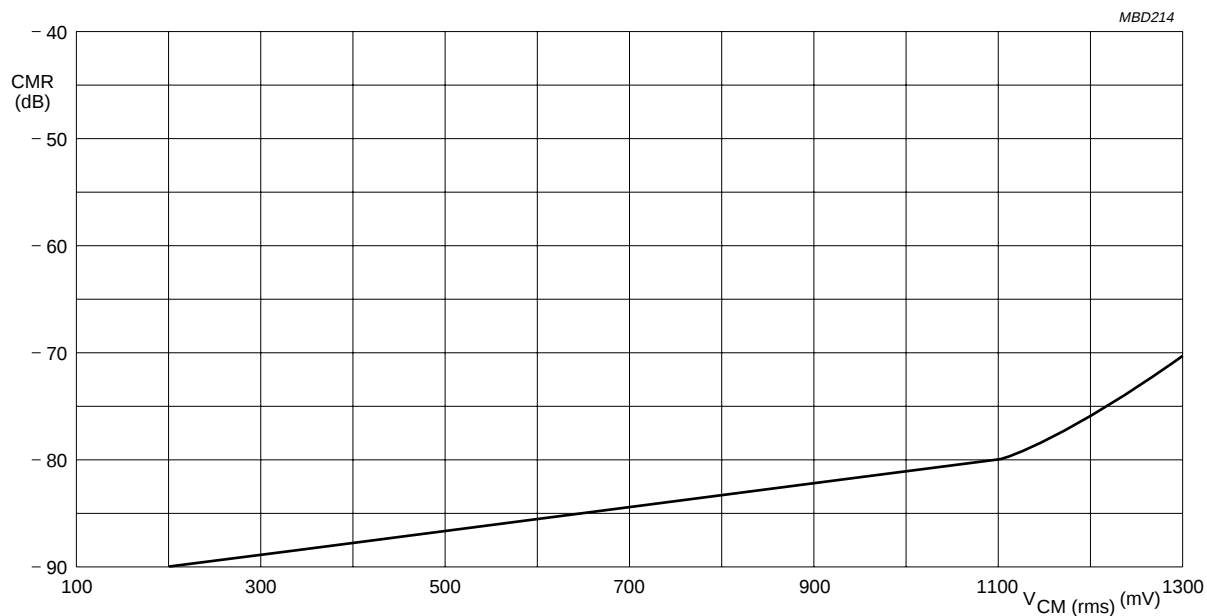
Fig.7 Common-mode rejection ratio as a function of common-mode input voltage; f = 1 \text{ kHz} ( R_s = 0 \Omega ).
