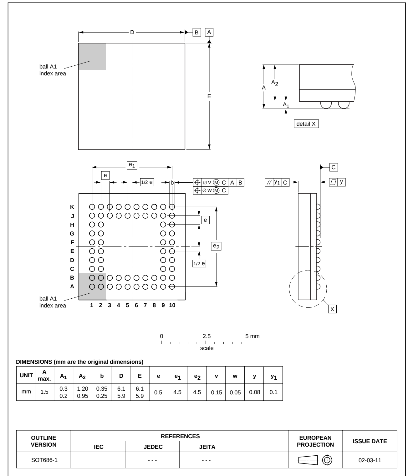
LFBGA64: plastic low profile fine-pitch ball grid array package; 64 balls; body 6 x 6 x 1.05 mm SOT686-1
