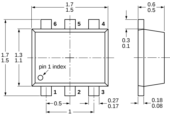
Fig 10. Package outline PEMH2 (SOT666)
