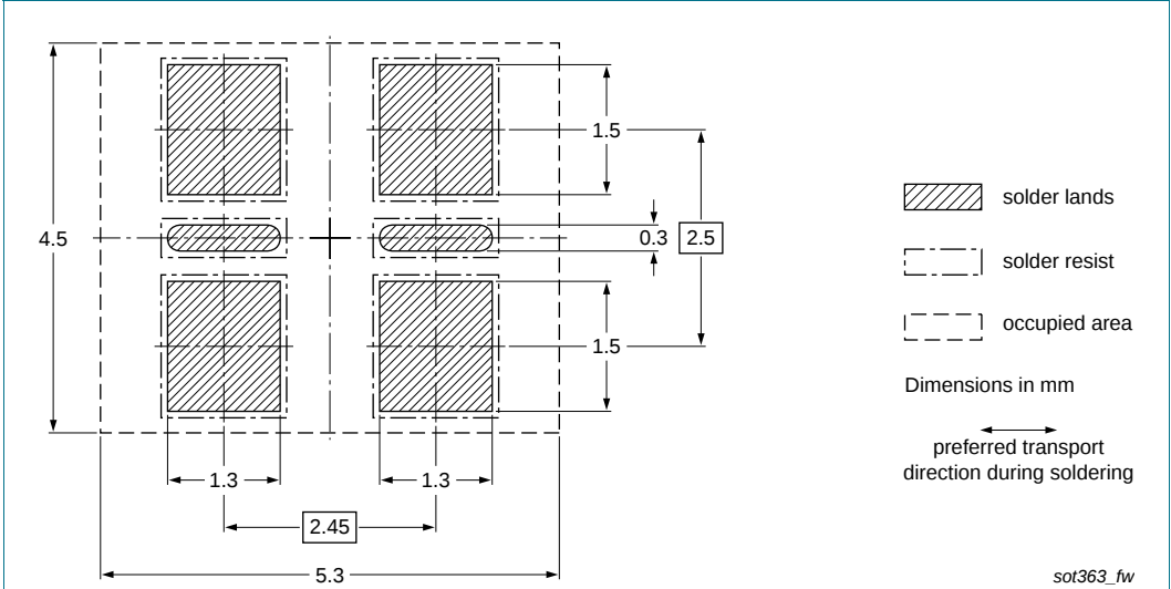
Fig 14. Wave soldering footprint PUMH2 (SOT363)
