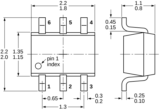
Fig 11. Package outline PUMH2 (SOT363)
