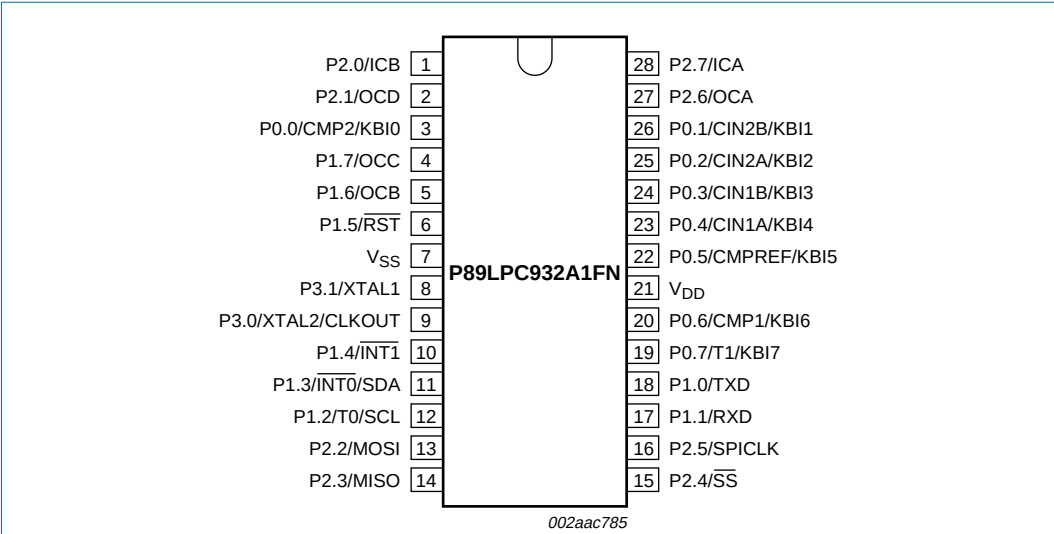
Fig 6. P89LPC932A1 DIP28 pin configuration
