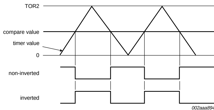
Fig 10. Symmetrical PWM
