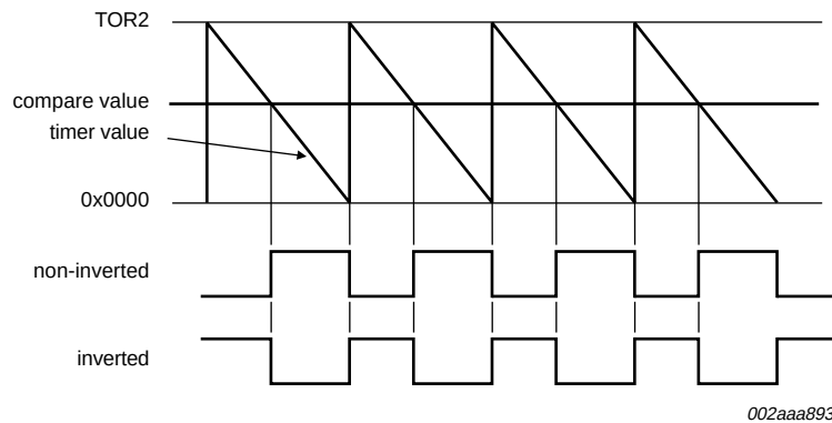
Fig 9. Asymmetrical PWM, down-counting
