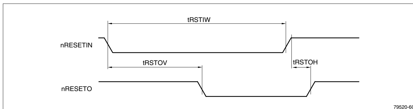
Figure 30. External Reset
