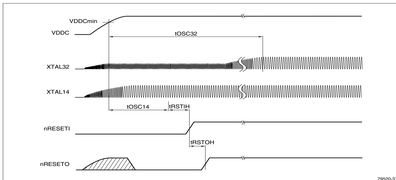
Figure 29. PLL Start-up
