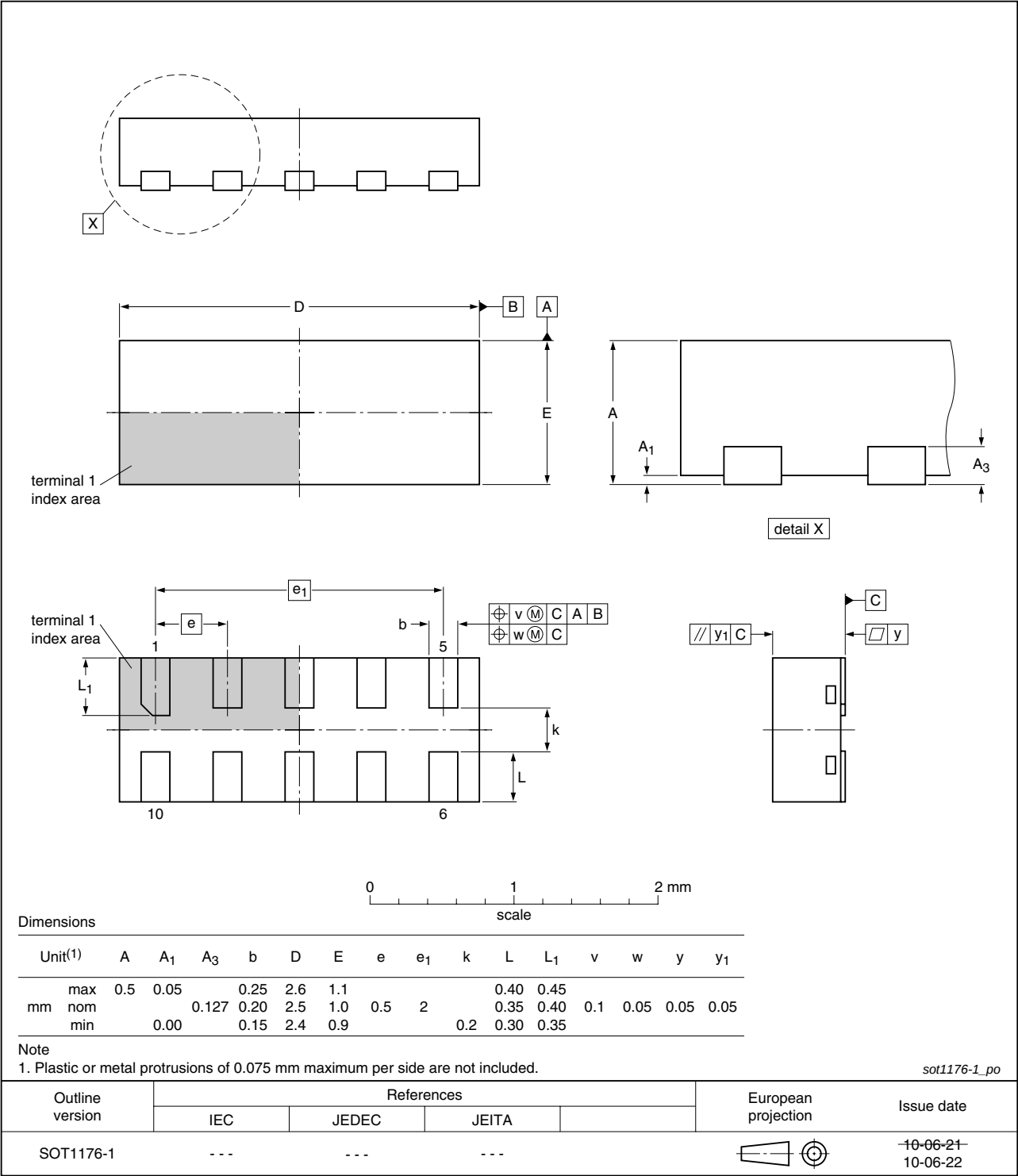
Fig 12. Package outline SOT1176-1 (XSON10)
