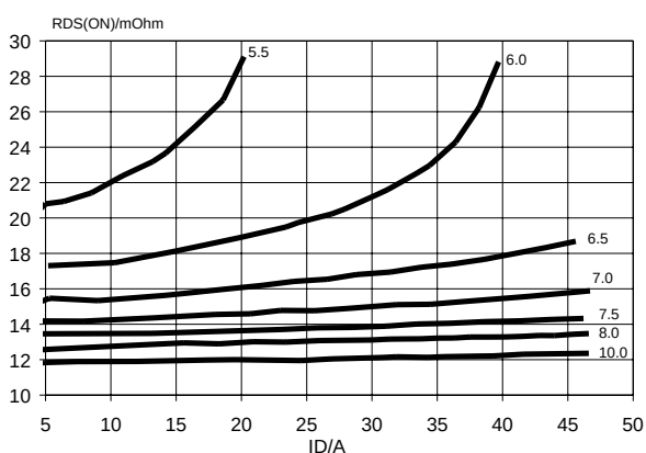
Fig.6. Typical on-state resistance, T_j = 25\text{ °C} . R_{DS(ON)} = f(I_D) ; parameter V_{GS}
