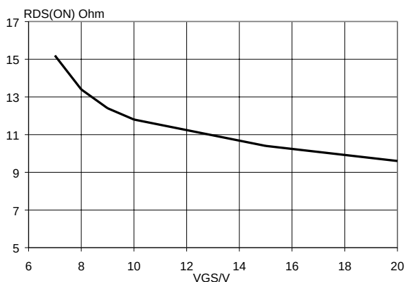
Fig.7. Typical on-state resistance, T_j = 25\text{ °C} . R_{DS(ON)} = f(V_{GS}) ; conditions: I_D = 25\text{ A} ;
