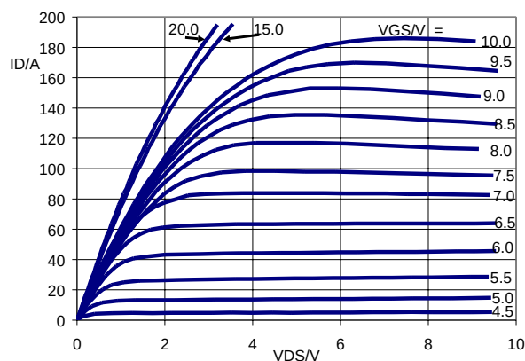
Fig.5. Typical output characteristics, T_j = 25\text{ °C} . I_D = f(V_{DS}) ; parameter V_{GS}
