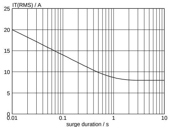
Fig.5. Maximum permissible repetitive rms on-state current I_{T(RMS)} , versus surge duration, for sinusoidal currents, f = 50 Hz; T_{hs} \leq 73^\circ\text{C} .
