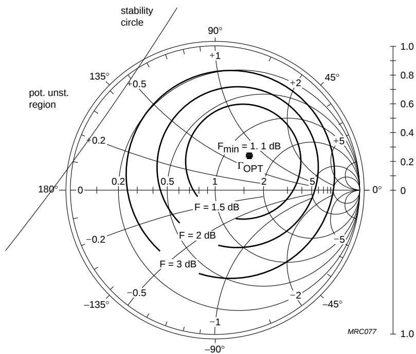
Fig.12 Noise circle.
