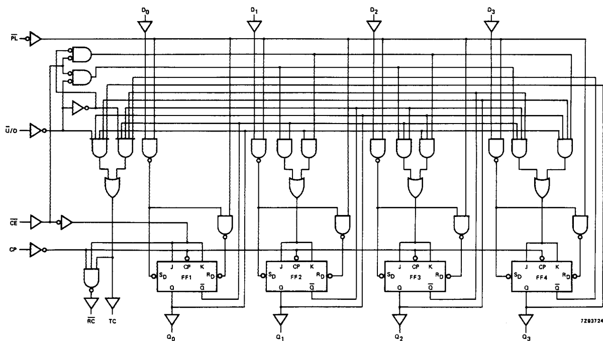
Fig.9 Logic diagram.
