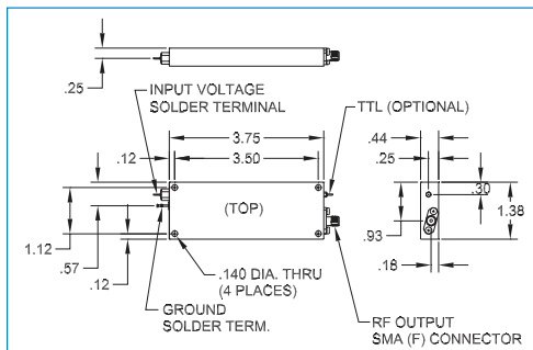
NC1000 Series Dimensions - Package 3 (inches)
