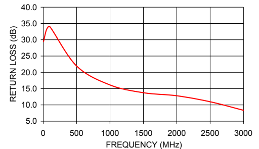
TC1-1-13M-75+ INPUT RETURN LOSS
