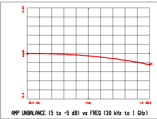
Amplitude Unbalance
