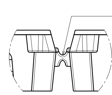
Snapping point * Detail A Scale: 4:1
