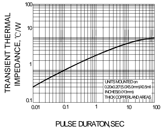
FIG.6-TRANSIENT THERMAL IMPEDANCE
