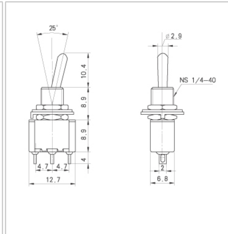
KLS7-MS-103-A1 ON-OFF-ON KLS7-MS-113-A1 ON-OFF-(ON) KLS7-MS-123-A1 (ON)-OFF-(ON)
