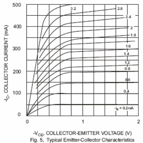
Fig. 5, Typical Emitter-Collector Characteristics
