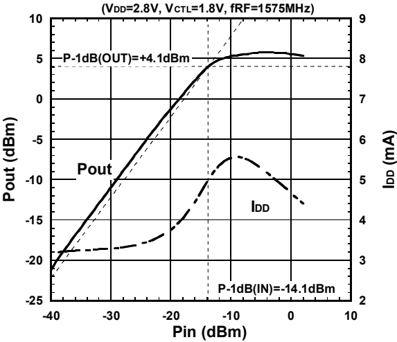
Pout, I DD vs. Pin
