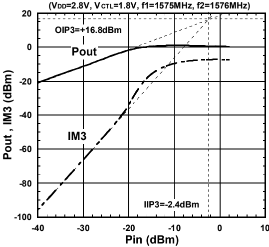
Pout, IM3 vs. Pin
