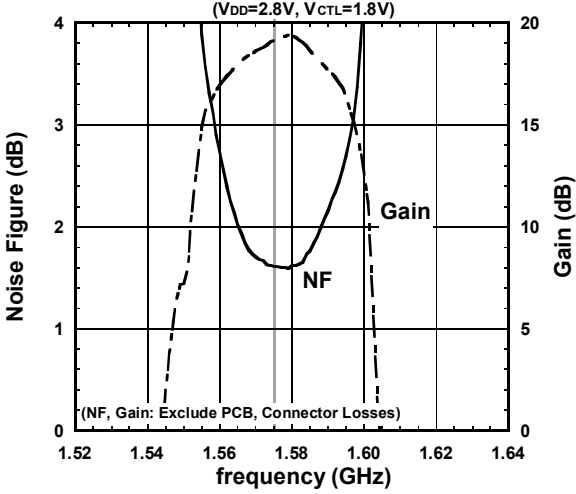
NF, Gain vs. frequency
